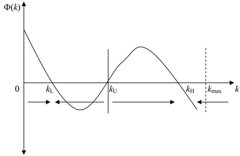
Figure 5: Global Stability
