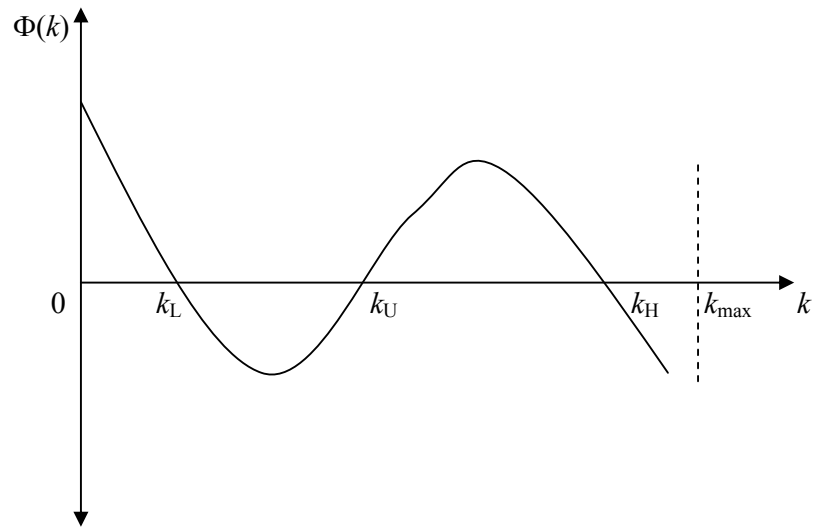
Figure 4: \Phi(k)
